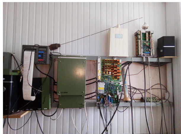
Picture 4. MF/HF units with NAVTEX (Real equipment)
